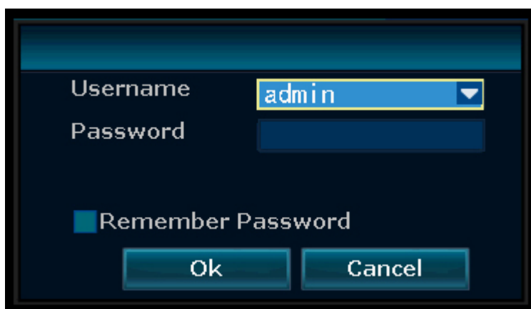
Illustration 3: Log in
